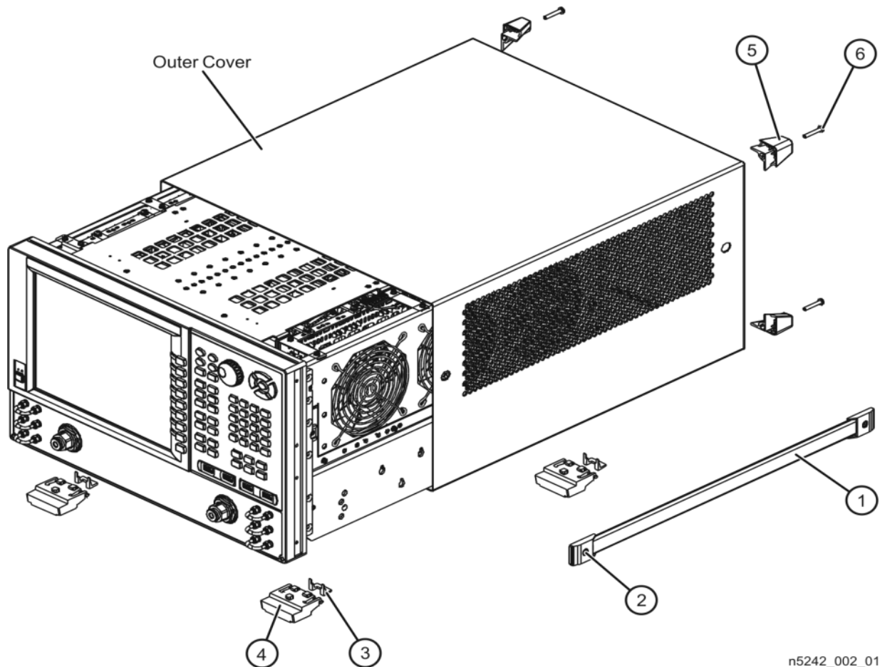
Figure 17 Outer Cover Reinstallation
