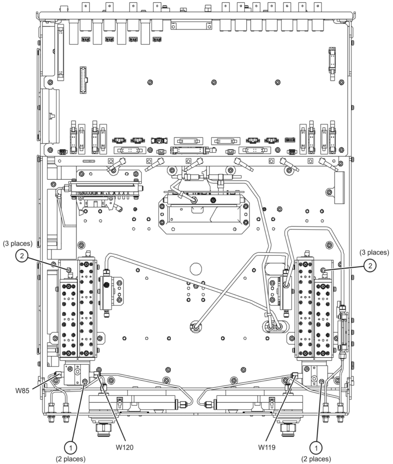
Figure 4 Existing Attenuators and Brackets Removal
