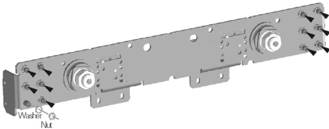
Figure 11 Bulkhead Connectors Installation
