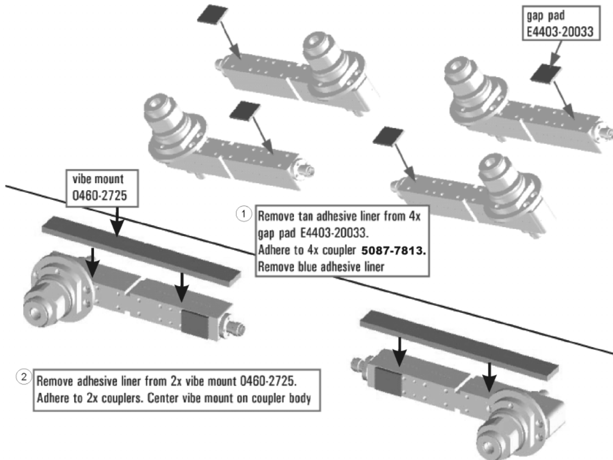
Figure 7 A29 and A32 Test Port Coupler Assembly
