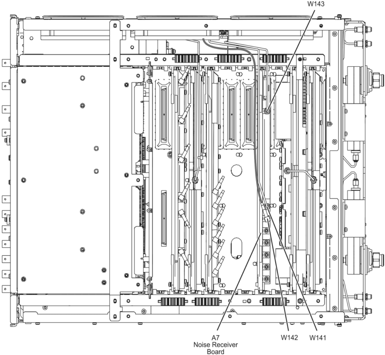
Figure 12 New Test Set Cable Installation, Part 2
