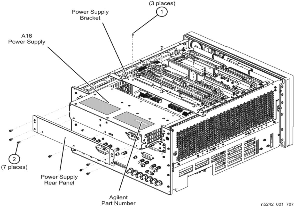
Figure 13 Power Supply Replacement
