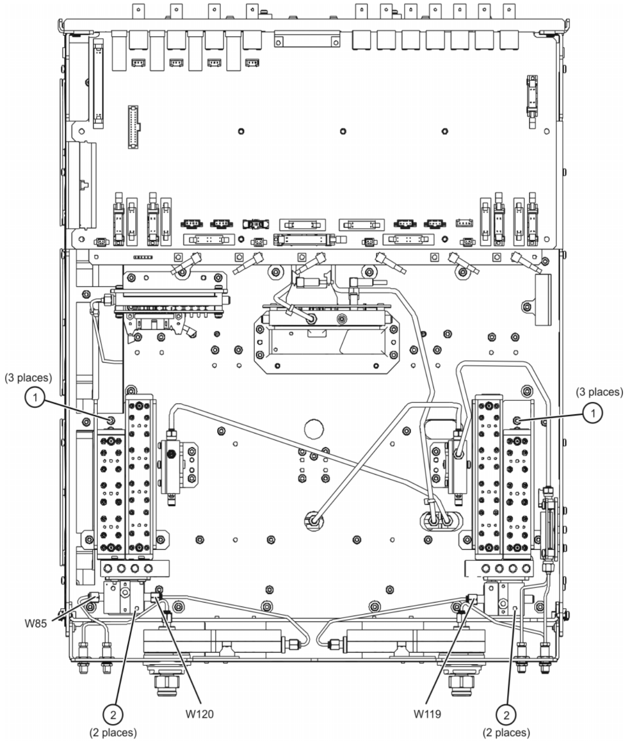
Figure 6 New Brackets Installation into the Analyzer
