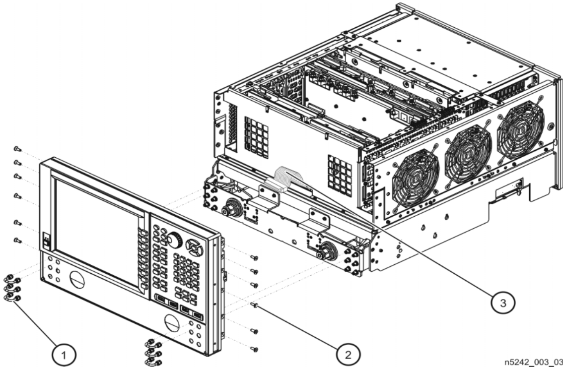
Figure 3 Front panel Assembly Removal
