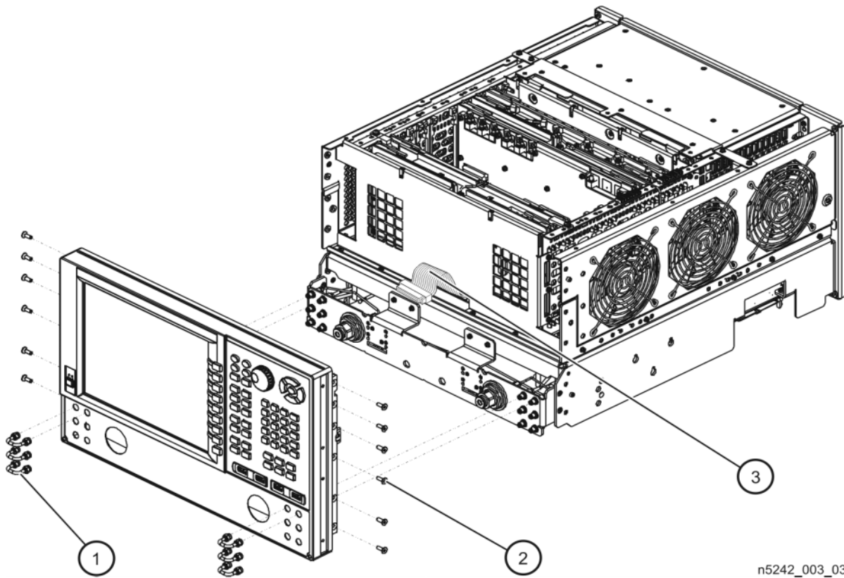
Figure 15 Front Panel Assembly Reinstallation
