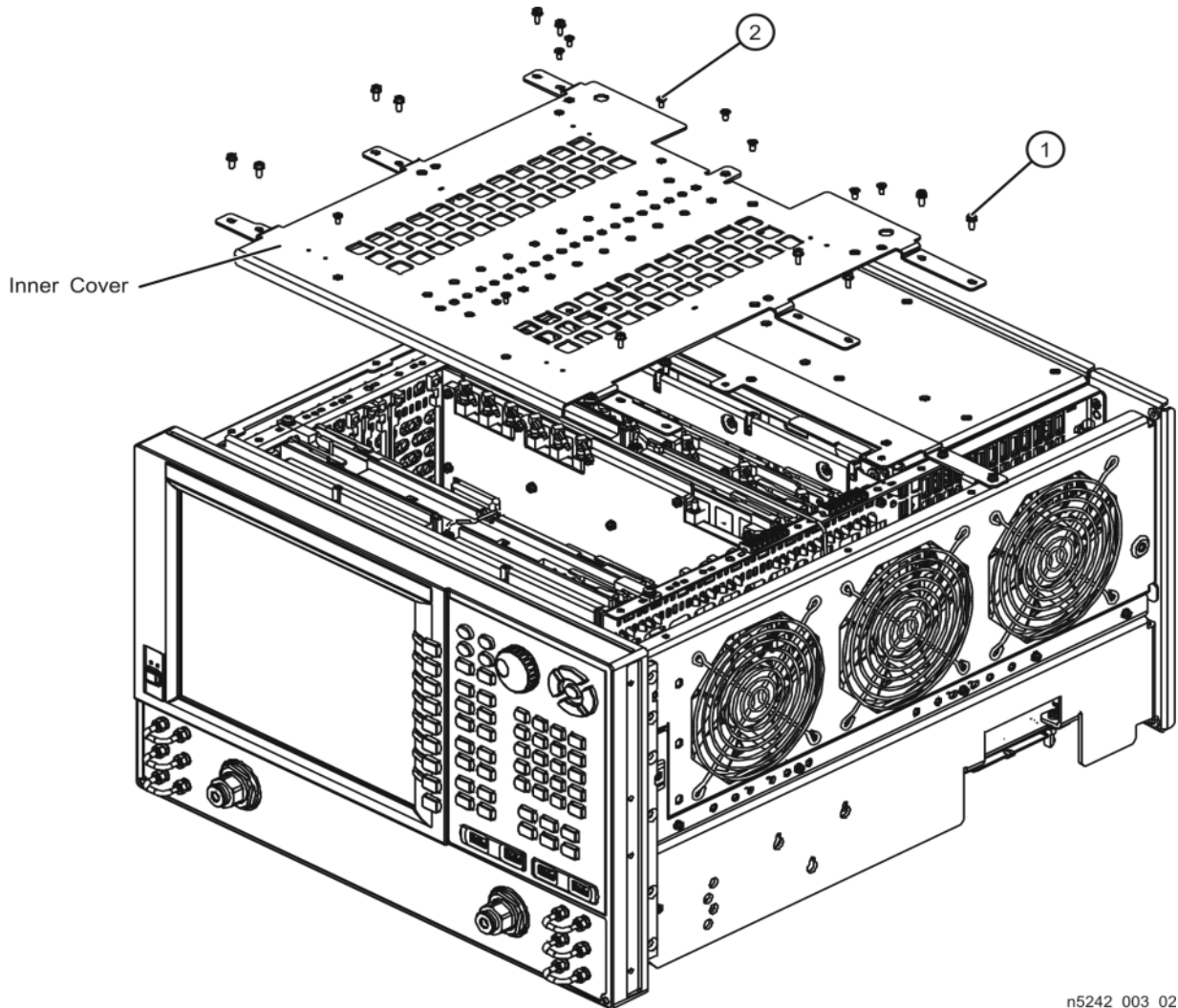
Figure 16 Inner Cover Reinstallation
