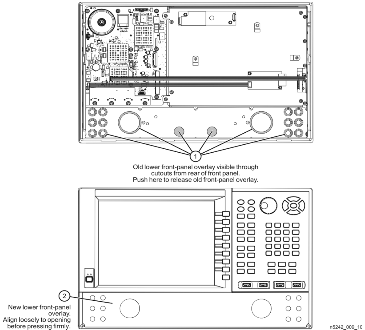
Figure 14 Lower Front panel Overlay Replacement
