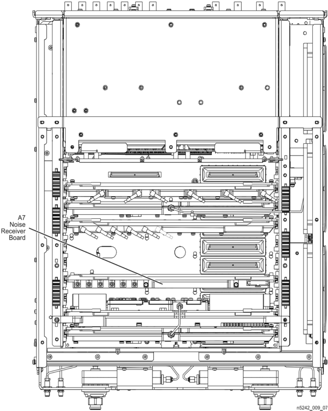
Figure 10 Noise Receiver Board Installation
