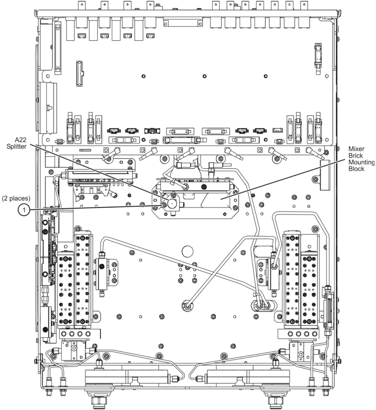
Figure 9 A22 Splitter Installation
